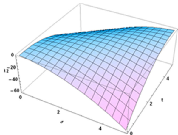
Figure 5. The 3D graphic for the \varpi_2(v, t) analytical solution (5) of Equations (1) for \varpi_1 = 1.8 , Q = 0.5 , c_1 = c_2 = 1 .
