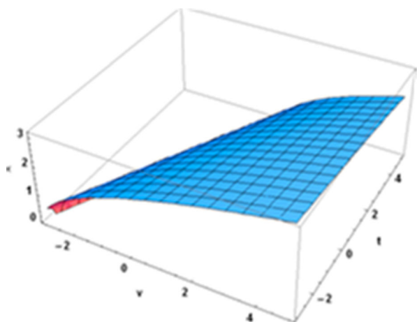
Figure 4. The 3D graphic for the \epsilon(v, t) analytical solution (5) of Equations (1) for \varpi_1 = 1.8 , Q = 0.5 , c_1 = 1 .
