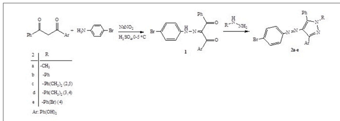
Figure 2. Synthesis of 1 and 2a-e .
