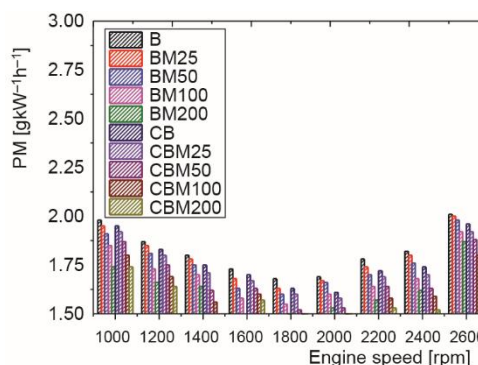
Figure 7. Change of PM emission value (for color image see journal web site)
