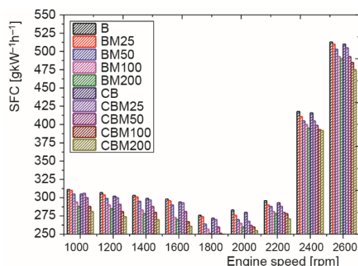
Figure 2. Change of the SFC value (for color image see journal web site)
