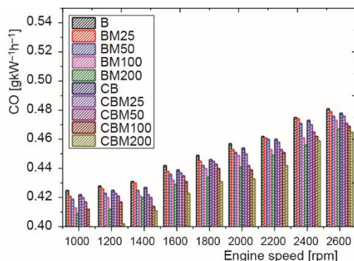
Figure 4. Change of CO emission value (for color image see journal web site)
