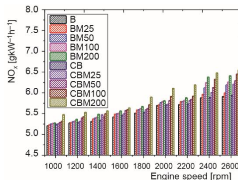
Figure 6. Change of \text{NO}_x emission value (for color image see journal web site)
