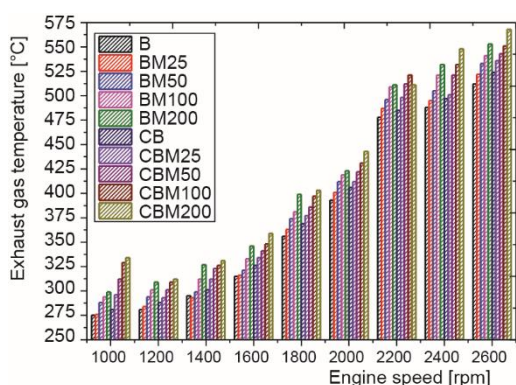
Figure 3. Variation of exhaust gas temperature (for color image see journal web site)
