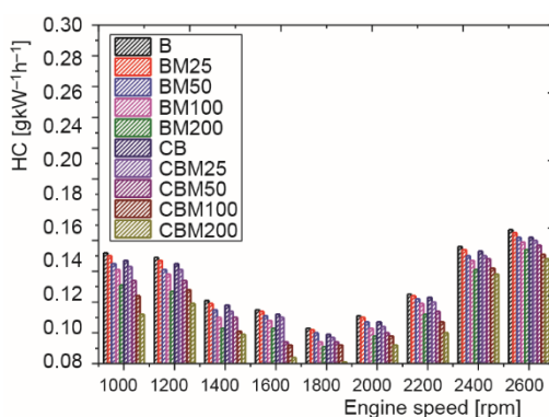
Figure 5. Change of HC emission value (for color image see journal web site)
