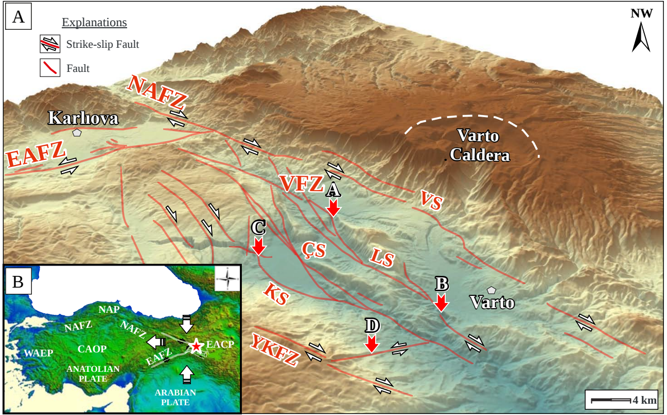
Figure 1. a) Digital elevation model of Varto region with main fault segments (A: Güzelkent geothermal field, B: Alagöztepe geothermal field, C: Kaynarca geothermal field, D: Karamiş mineral water, VS: Varto Segment, LS: Leylekdağ Segment, ÇS: Çayçatı Segment, KS: Kaynarca Segment, YKFZ: Yorgançayır-Kaynarca Fault Zone), b) location map of the study area with major neotectonic structures and tectonic provinces of the Anatolia (Bozkurt, 2001; WAEP: West Anatolian Extensional Province, CAOP: Central Anatolian Ova Province, EACP: East Anatolian Contractual Province, NAP: North Anatolian Province, NAFZ: North Anatolian Fault Zone, EAFZ: East Anatolian Fault Zone).
