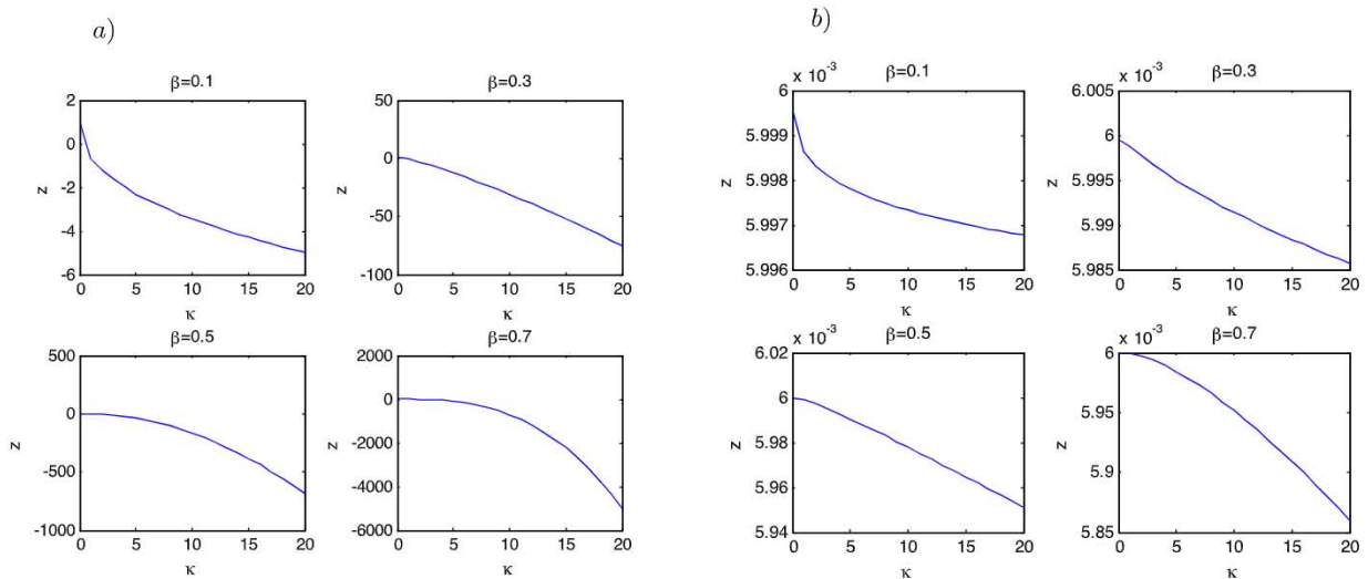
Fig. 2. The 2D graphics of the \tilde{z} ns with the help of ns of Eq. (1.1) for different values of \beta . a) RPSM , b) LS-RPSM ( \mu = 0.4 ).
