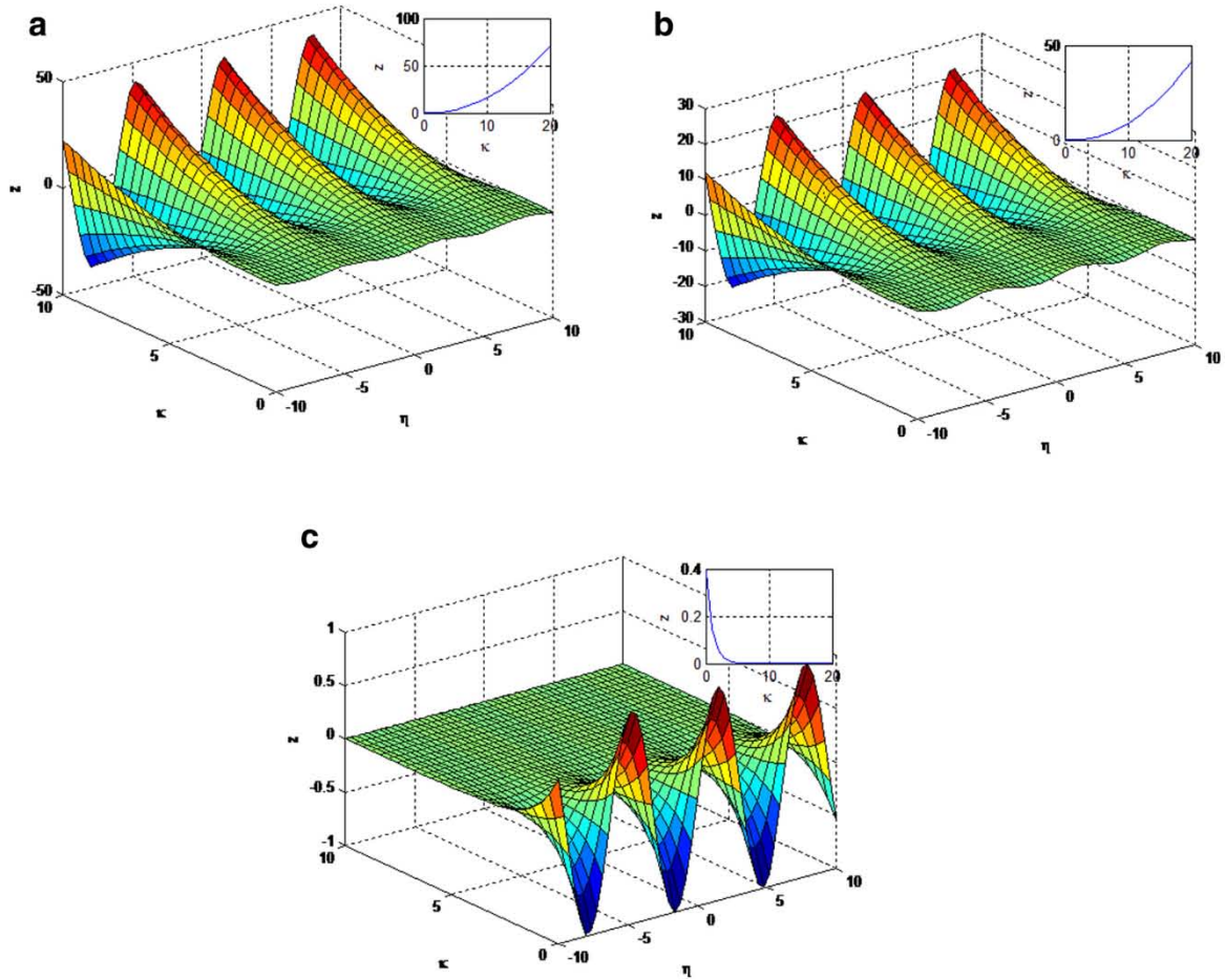
Fig. 5. 3D graphics for the ns with the help of RPSM, LS-RPSM and the exact solution of (1.3) equation a) (4.6) z numerical solution b) (4.27) z-tilde numerical solution c) The exact solution (beta = 1).
