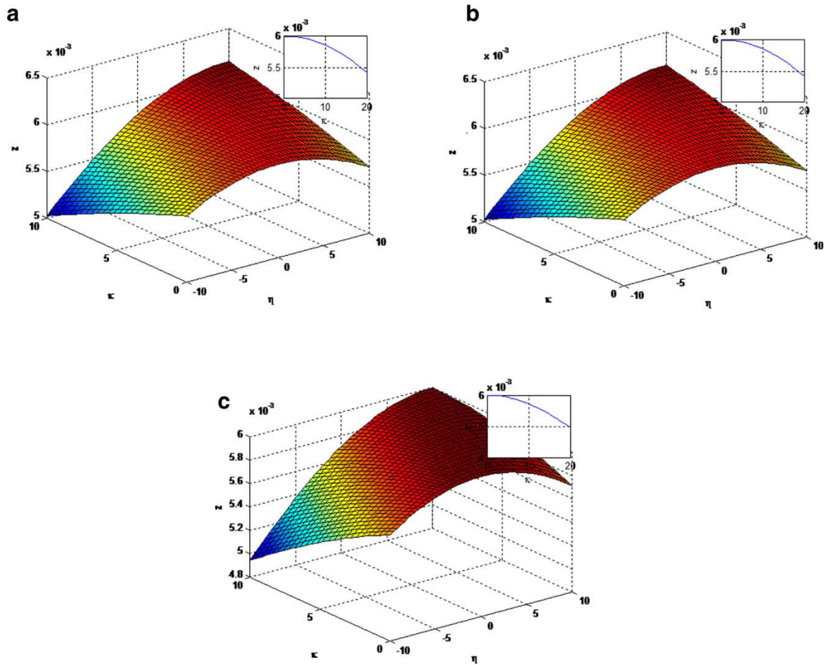
Fig. 1. 3D graphics for the ns with the help of RPSM, LS-RPSM and the es of Eq. (1.1) a) (4.2) z numerical solution B) (4.13) \tilde{z} numerical solution c) The exact solution ( \beta = 1, a = 0.02 ).
