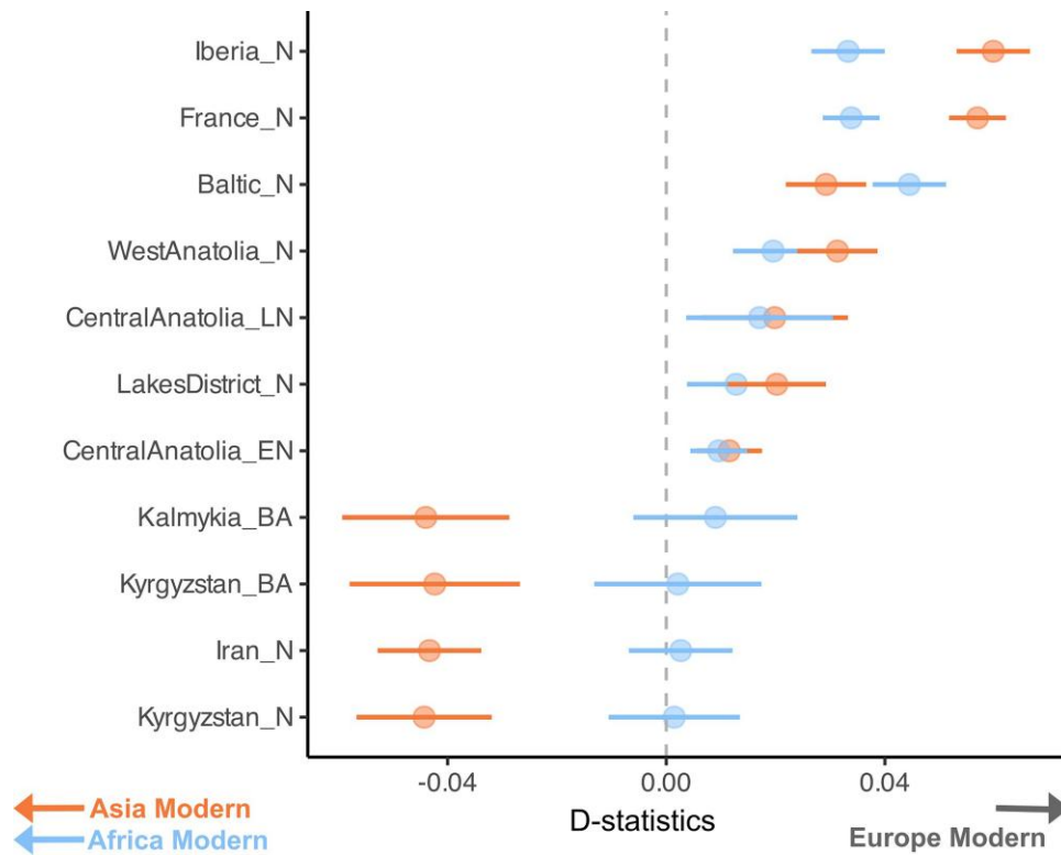
Fig. 4. D -statistics of the form D(\text{Goat, Anatolian/Asian/European ancient; non-EU, EU}) . EU, European modern-day breeds; non-EU, Asian and African modern-day breeds. The orange points show comparisons between modern-day European and Asian breeds, and the blue points show comparisons between modern-day European and African breeds. Positive values indicate ancient genomes showing higher affinity to EU, while negative values indicate higher affinity to non-EU. D -statistics were calculated with angsd (Korneliussen et al. 2014) using de novo variants. Error bars show \pm 3 standard errors (no multiple testing correction applied).
